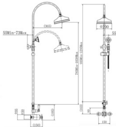
Belgravia Thermostatic Shower Set NV138 Flow Rates: 0.5 Bar 8.6 | 1 Bar 12 | 5 Bar 21.7
