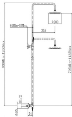
Islington Round Thermostatic Shower Set NV134 NV134-MB NV134-BB Flow Rates: 0.5 Bar 7.6 | 1 Bar 10.7 | 5 Bar 18.7
