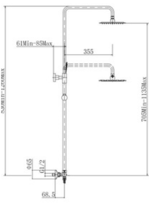
Westminster Thermostatic Shower Set NV13RS Flow Rates: 0.5 Bar 6.6 | 1 Bar 9.2 | 5 Bar 15.7
