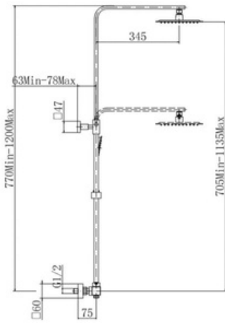
Mayfair Square Thermostatic Shower Set NV136 NV136-MB NV136-BB Flow Rates: 0.5 Bar 7.6 | 1 Bar 10.7 | 5 Bar 18.7
