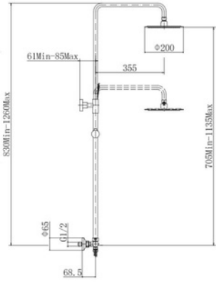
Lewisham Thermostatic Shower Set NV139R Flow Rates: 0.5 Bar 5 | 1 Bar 7.2 | 5 Bar 12.2
