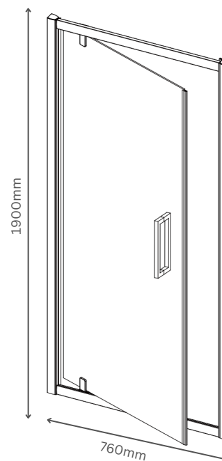
Dimensions (measurements in mm)
