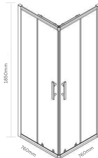
Dimensions (measurements in mm)
